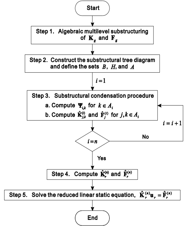
Fig. 3 Computational procedure of the automated static condensation method
