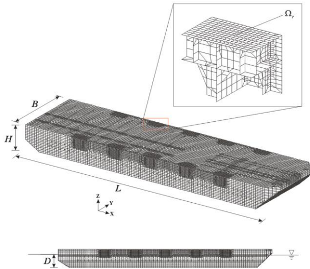
Fig. 6 Barge structure problem (123770 shell elements, Global model of 347604 DOFs, Retained substructure \Omega_r of 5268 DOFs)
