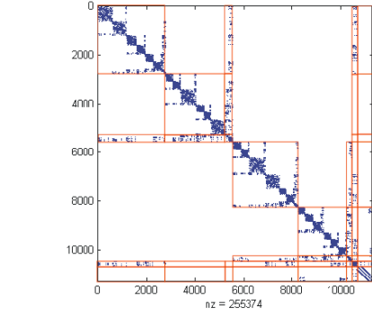
(a) Re-permuted and re-partitioned matrix
