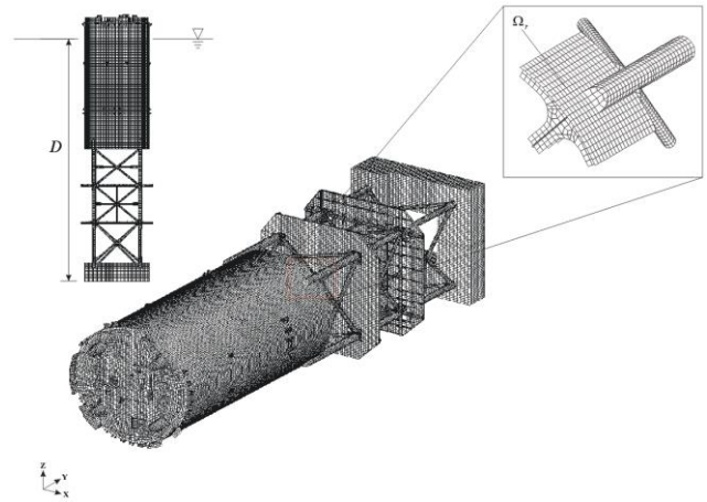
Fig. 7 Spar structure problem (337825 shell elements, Global model of 1831242 DOFs, Retained substructure \Omega_r of 18084 DOFs)
