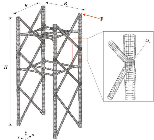
Fig. 5 Jacket structure problem (26484 shell elements, Global model of 155766 DOFs, Retained substructure \Omega_r of 6816 DOFs)
